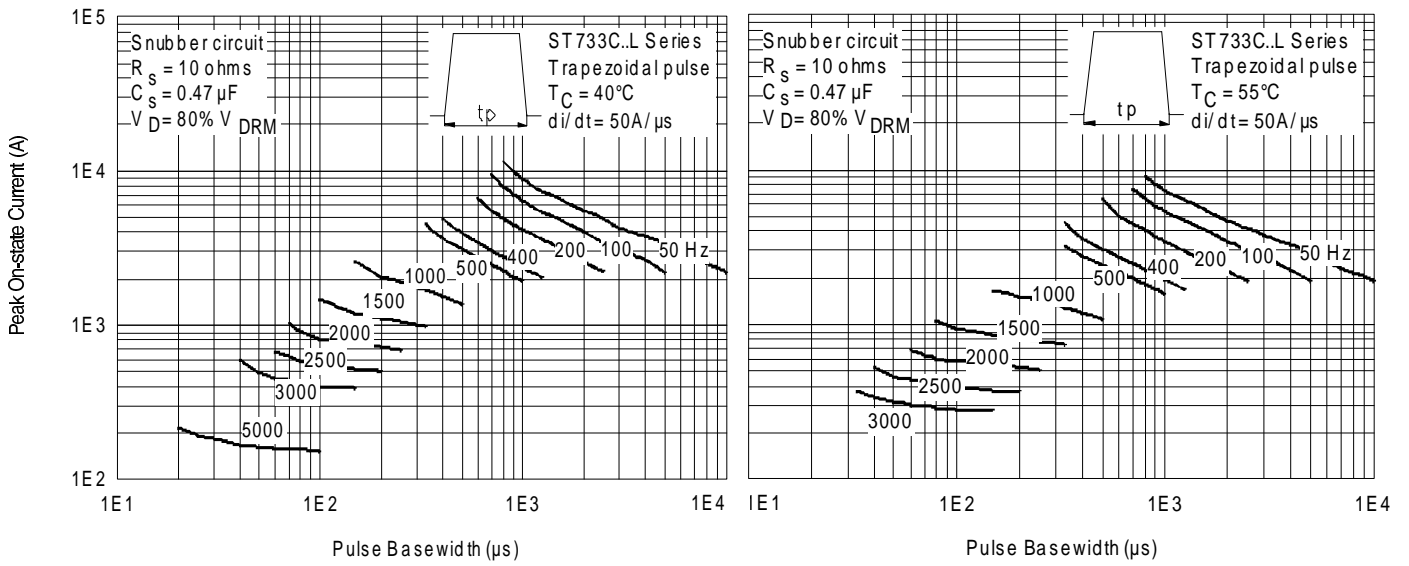
Fig. 14 - Frequency Characteristics
