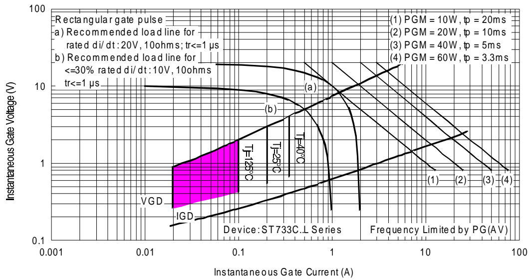
Fig. 17 - Gate Characteristics
