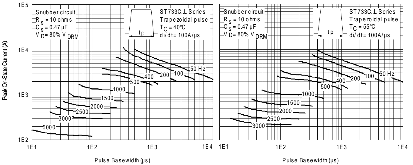
Fig. 15 - Frequency Characteristics
