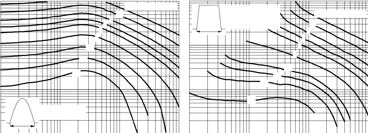
Fig. 15 - Frequency Characteristics
