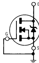
Figure 8b – V_{DS} Stress Equals 80% of B_{V_{DS}} During Radiation.
