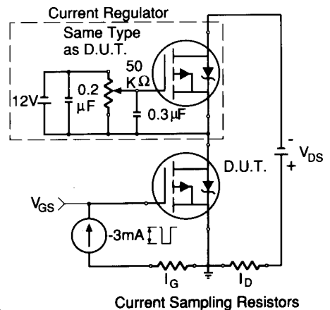
Fig. 13a — Gate Charge Test Circuit
