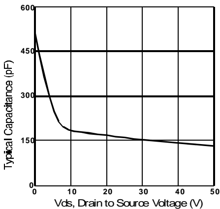
Figure 9. Typical Output Capacitance
