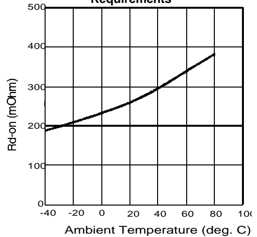
Figure 4. Typical On-Resistance
