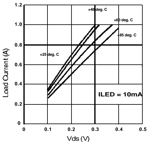
Figure 3. Typical On-Characteristics
