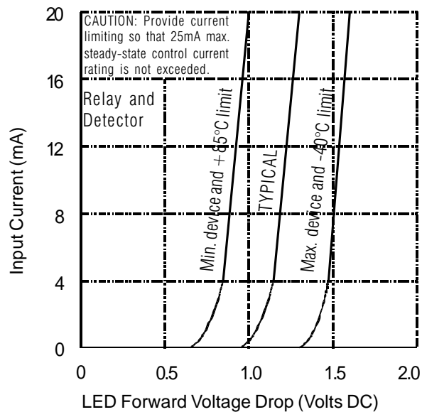
Figure 6. Input Characteristics (Current Controlled)
