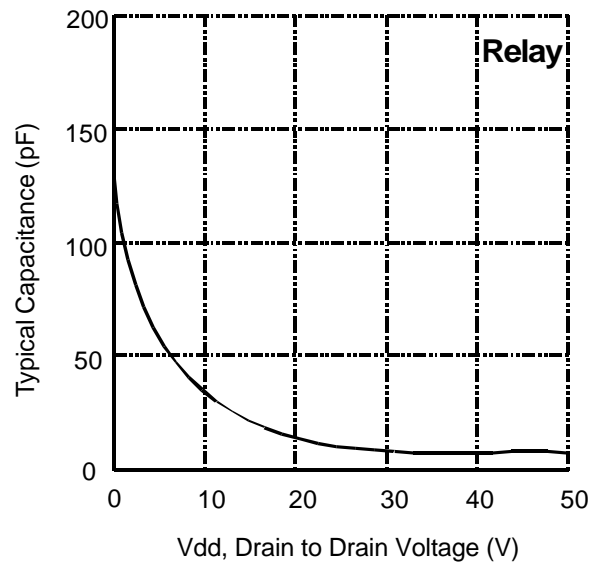
Figure 2. Typical Output Capacitance
