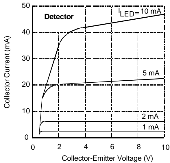
Figure 9. Typical Transfer Characteristics
