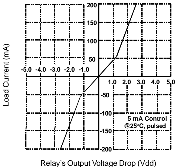
Figure 3. Linearity Characteristics
