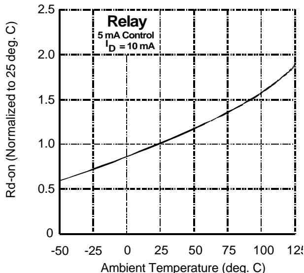
Figure 4. Typical Normalized On-Resistance
