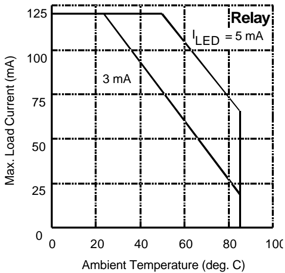
Figure 1. Current Derating Curve
