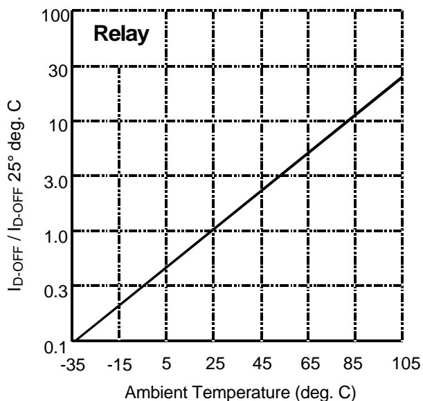
Figure 5. Typical Normalized Off-State Leakage
