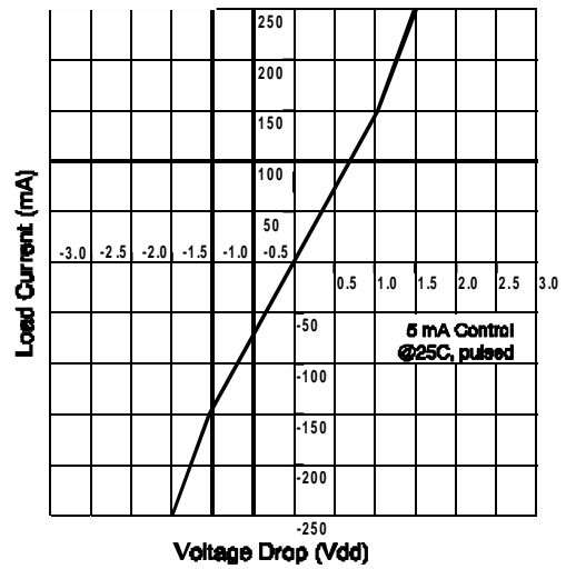
Figure 2. Linearity Characteristics
