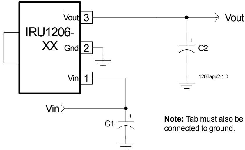
Figure 2 - Typical application of IRU1206.
