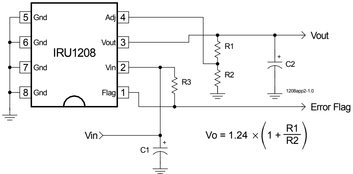
Figure 4 - Typical application of IRU1208 in 3.3V to 2.5V regulator.
