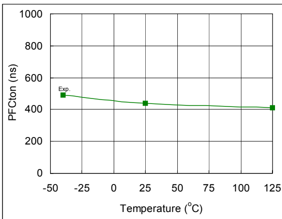
Fig. 58. Turn-On Propagation Delay vs. Temperature
