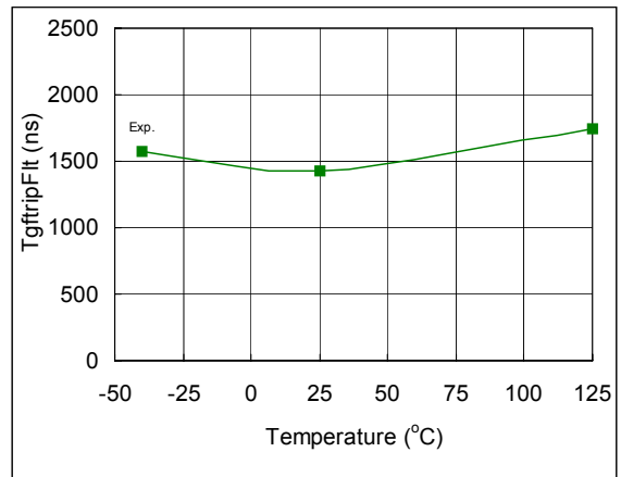
Fig. 77. GF TRIP to Fault Time vs. Temperature
