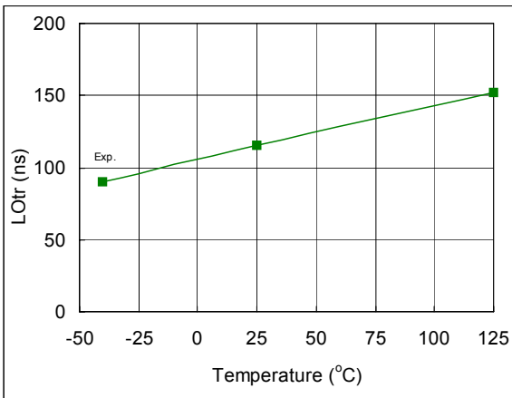
Fig. 52. Turn-On Rise Time vs. Temperature
