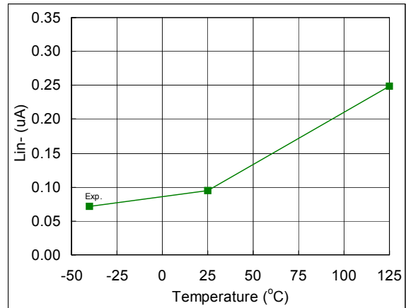
Fig. 41. Input Bias Current vs. Temperature
