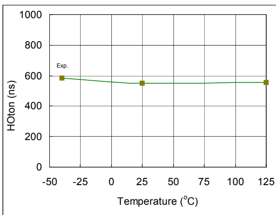
Fig. 54. Turn-On Propagation Delay vs. Temperature
