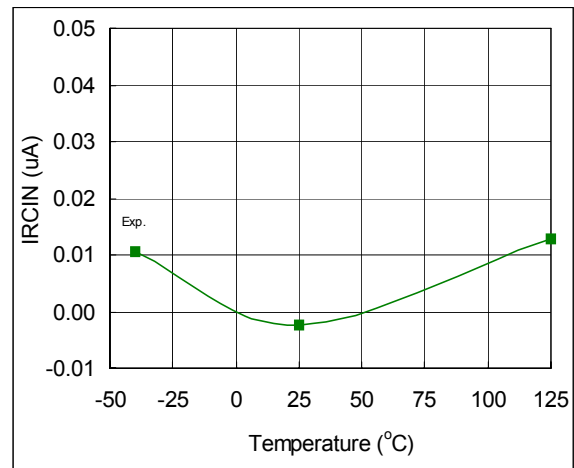
Fig. 43. RCIN Input Bias Current vs. Temperature
