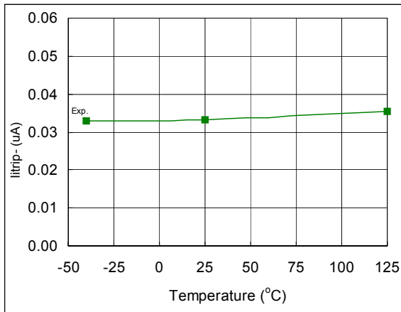
Fig. 46. ITRIP Input Bias Current vs. Temperature
