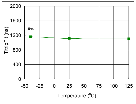
Fig. 67. ITRIP to Fault Time vs. Temperature
