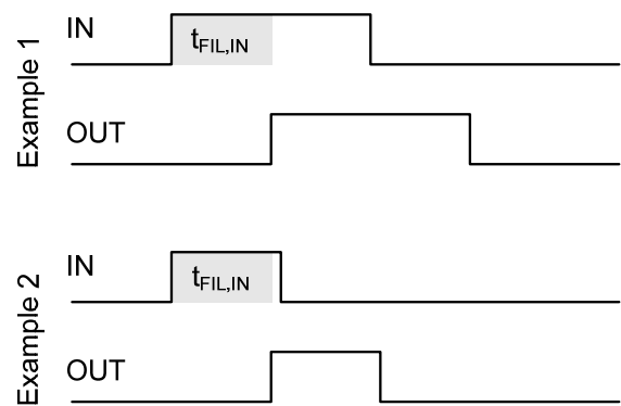
Figure 20: Advanced input filter
