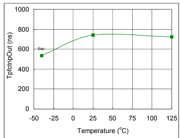
Fig. 73. PFC TRIP to Output Shutdown Propagation Delay
