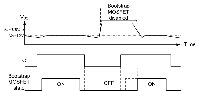
Figure 25: Bootstrap MOSFET state diagram
