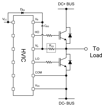
Figure 38: V_S resistor
