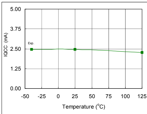
Fig. 48. Quiescent V CC Supply Current vs. Temperature
