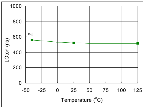
Fig. 50. Turn-On Propagation Delay vs. Temperature
