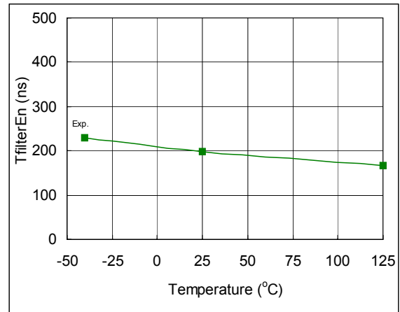
Fig. 83. Enable Input Filter Time vs. Temperature
