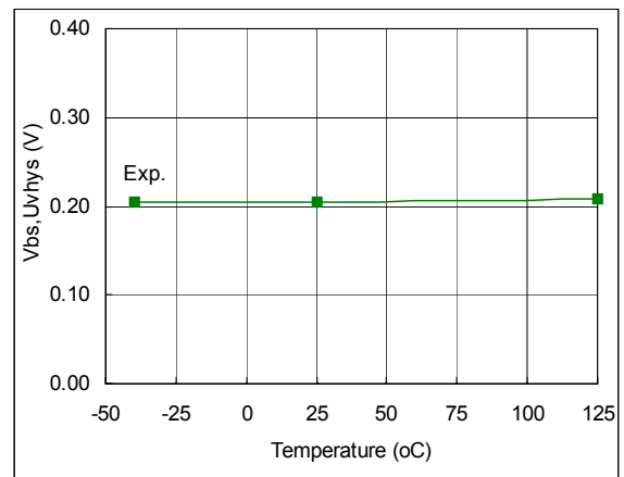
Fig. 107. V BS Supply Undervoltage Hysteresis vs. Temperature
