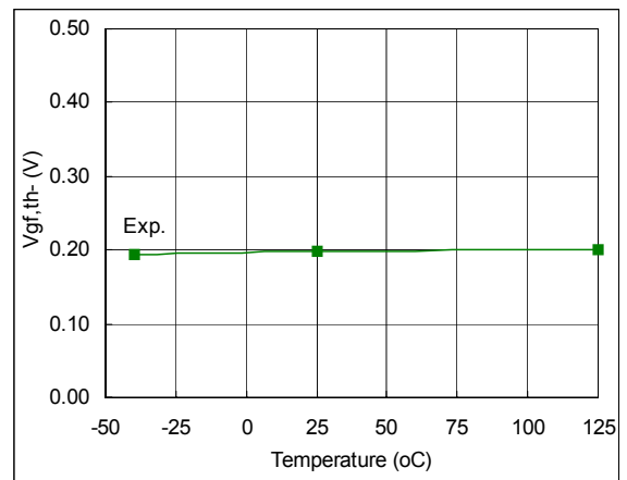
Fig. 101. GF Negative Going Threshold vs. Temperature
