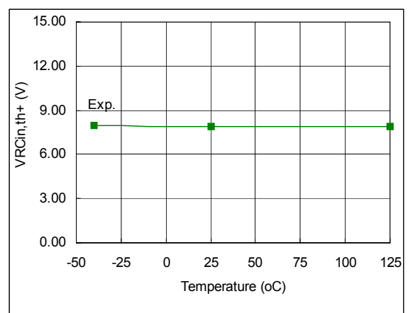
Fig. 103. RCIN Positive Going Threshold vs. Temperature
