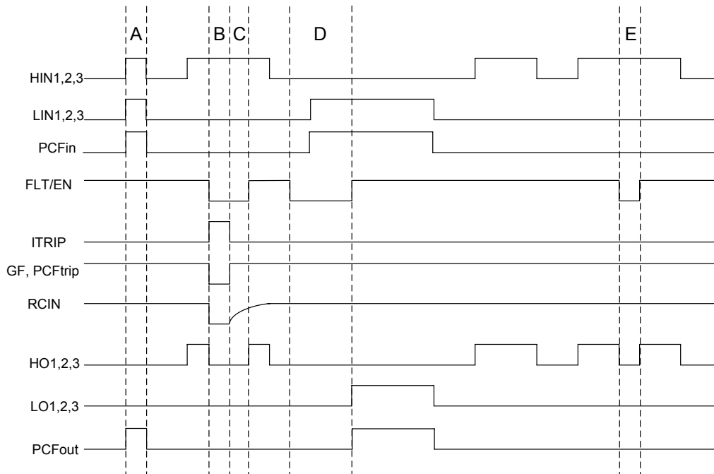
Figure 4: Input/output timing diagram
