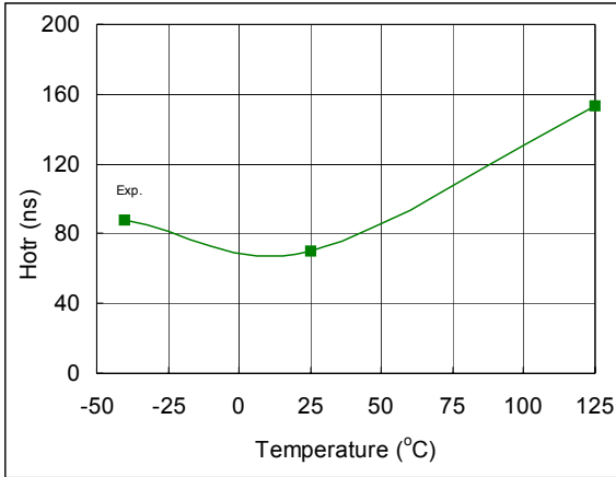
Fig. 56. Turn-On Rise Time vs. Temperature
