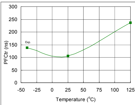
Fig. 60. Turn-On Rise Time vs. Temperature
