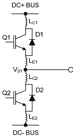
Figure 32: Parasitic Elements
