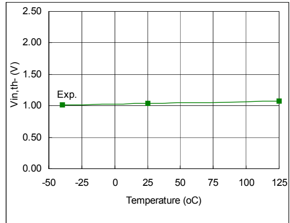
Fig. 95. Input Negative Going Threshold vs. Temperature
