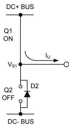
Figure 28: Q1 conducting
