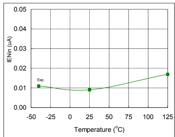
Fig. 115. En Input Bias Current vs. Temperature
