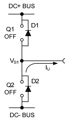
Figure 29: D2 conducting
