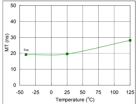
Fig. 63. Ton, Off Matching Time vs. Temperature
