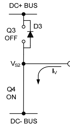
Figure 31: Q4 conducting
