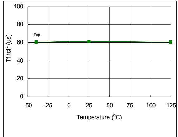
Fig. 75. FAULT Clear Time RCIN vs. Temperature
