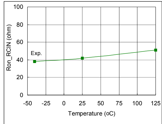
Fig. 93. RCIN Low On Resistance vs. Temperature
