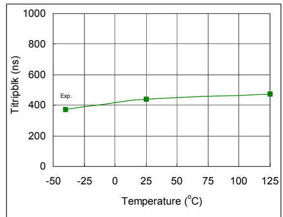
Fig. 71. ITRIP Blanking Time vs. Temperature
