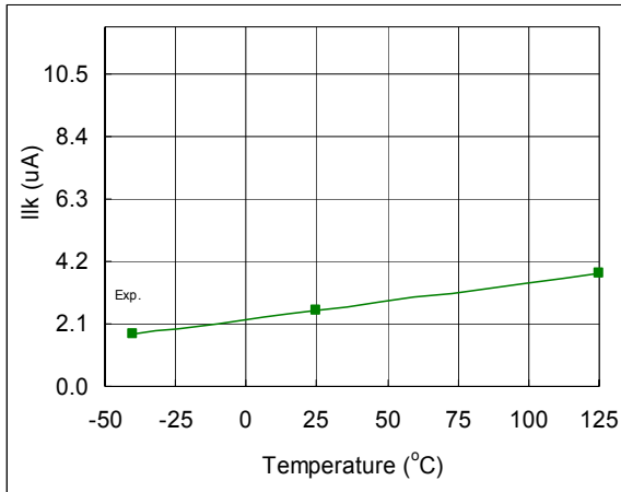
Fig. 40. Offset Supply Leakage Current vs. Temperature
