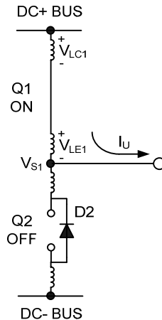
Figure 33: V_S positive
