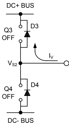
Figure 30: D3 conducting
