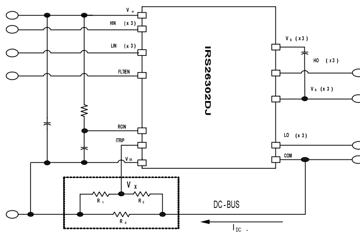
Figure 37: Supply capacitor
