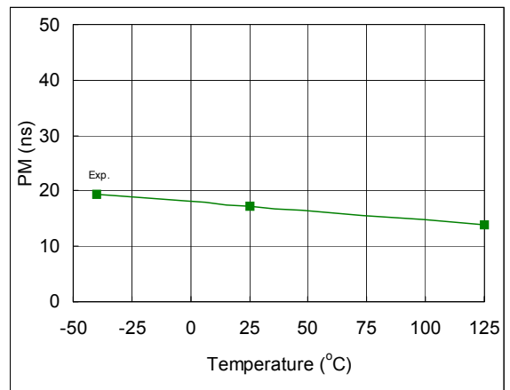
Fig. 65. Pulse Width Distortion vs. Temperature
