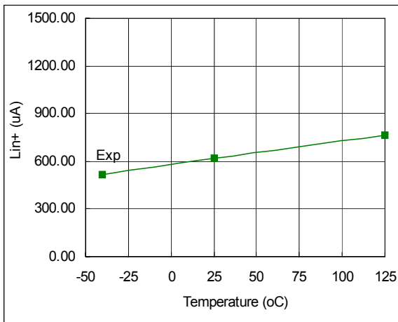
Fig. 42. Input Bias Current vs. Temperature
