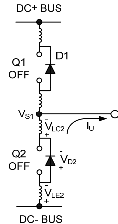
Figure 34: V_S negative
