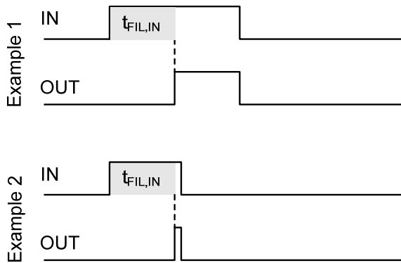
Figure 19: Typical input filter
