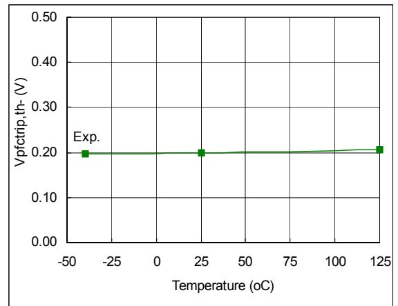
Fig. 99. PFC Negative Going Threshold vs. Temperature
