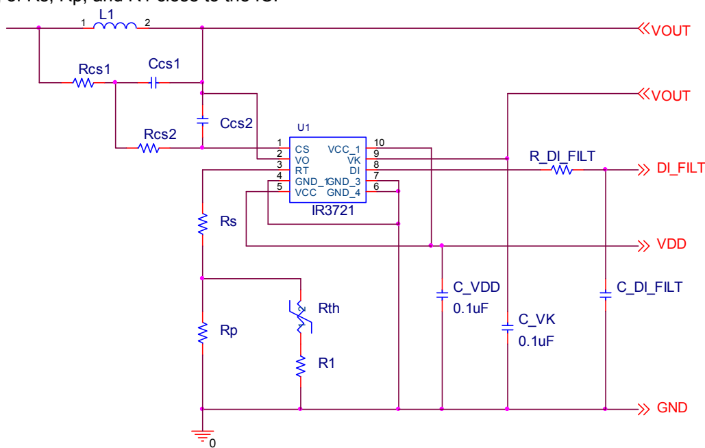
Figure 7 Example schematic
