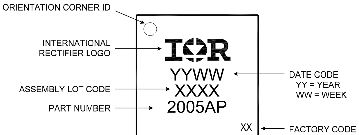
Figure 17 Part Marking
