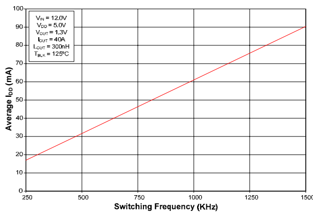
Figure 7 V_{DD} Supply Current vs. Switching Frequency
