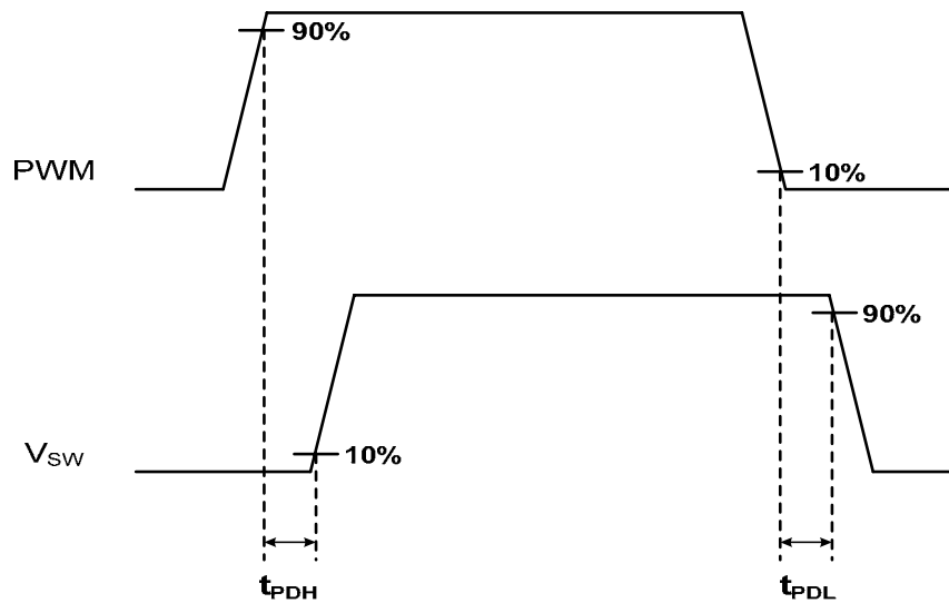
Figure 9 Timing Diagram
