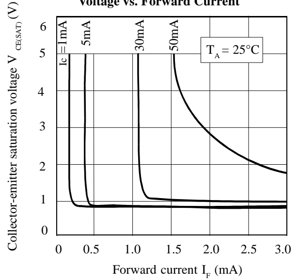
Collector-emitter Saturation Voltage vs. Forward Current
