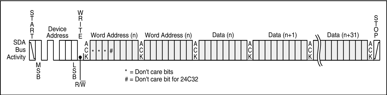
Figure 7. Page Write
