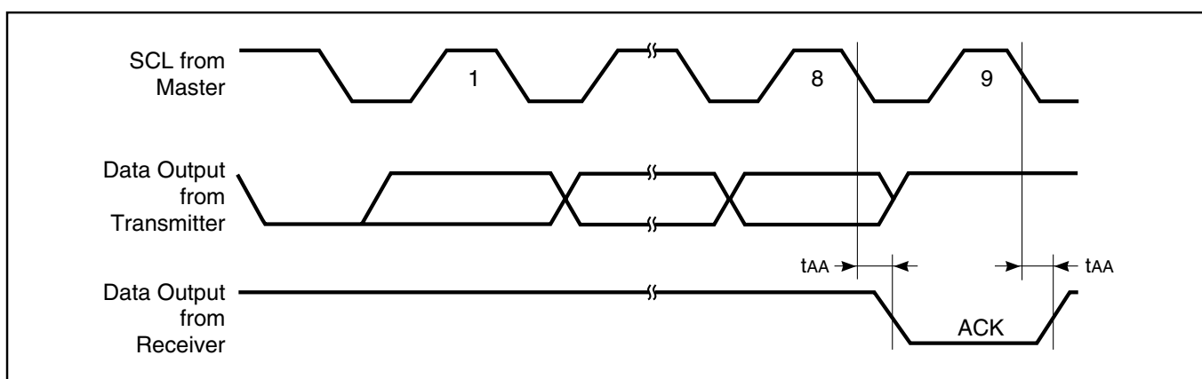
Figure 2. Output Acknowledge
