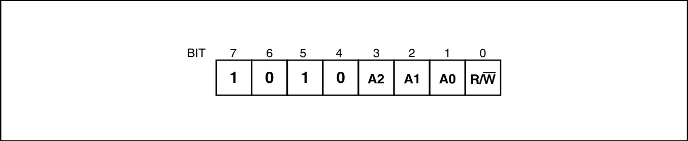
Figure 5. Slave Address
