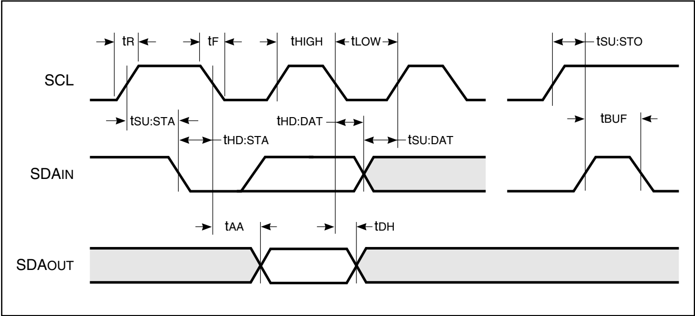
Figure 11. Bus Timing
