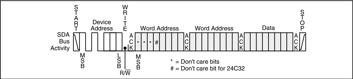
Figure 6. Byte Write
