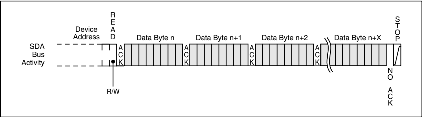
Figure 10. Sequential Read
