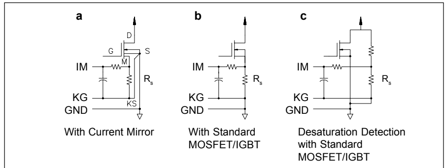
Fig. 8: Alternative overcurrent protection circuits
