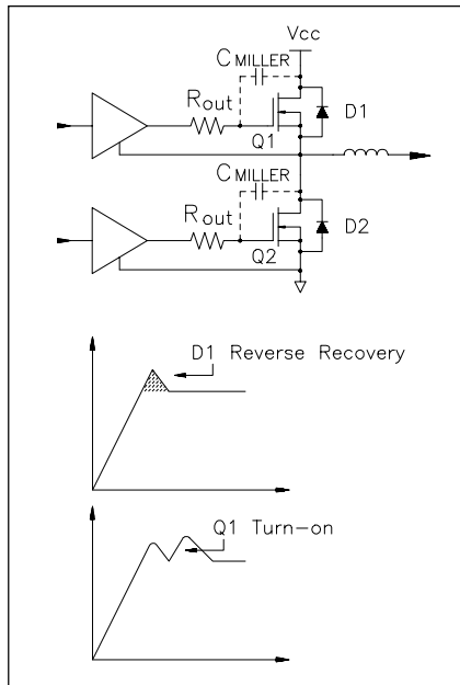
Fig. 6: Switching a clamped inductive load
