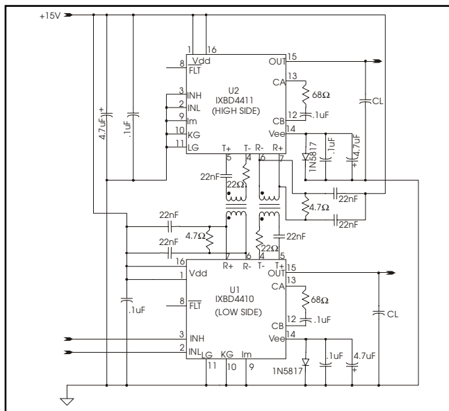
Fig. 2a: IXBD4410/4411 Switching time test circuit
