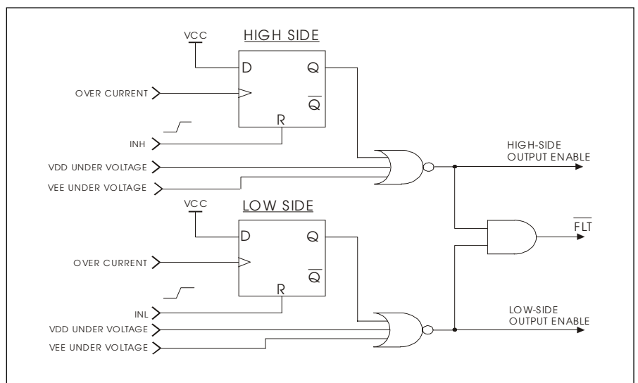
Fig. 5: Logic Representation of IXBD4410 FLT Signal
