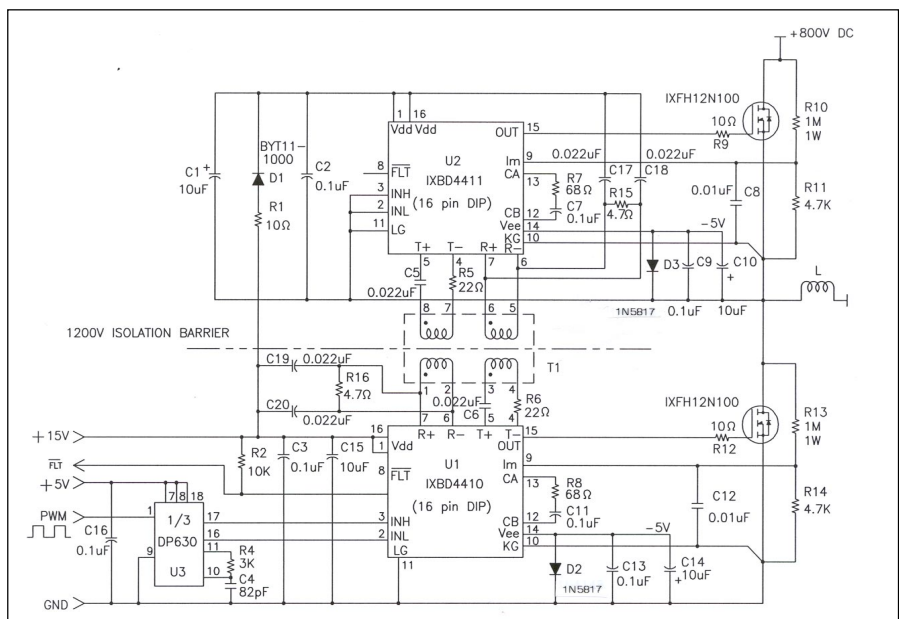
Fig. 7: IXBD4410/4411 Detailed one phase circuit with dead time generator IXDP 630
