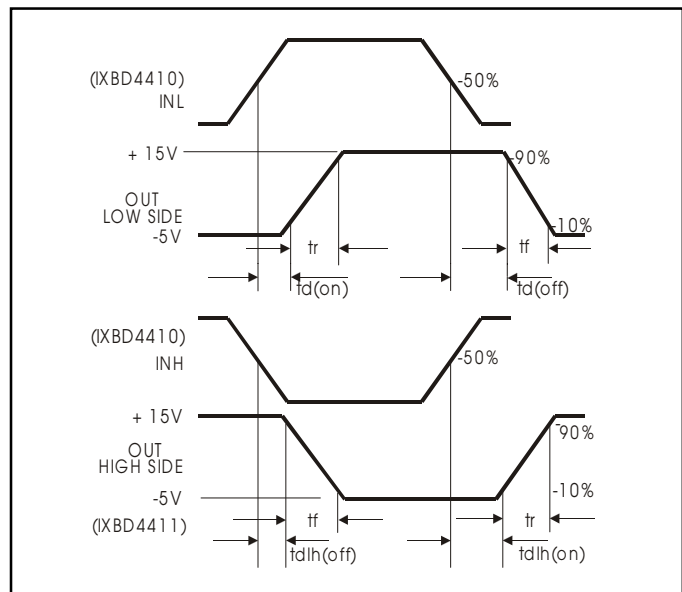
Fig. 2b: Output signal waveform
