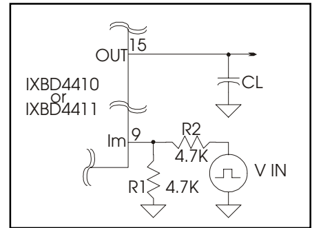
Fig. 1a Overcurrent Detection
