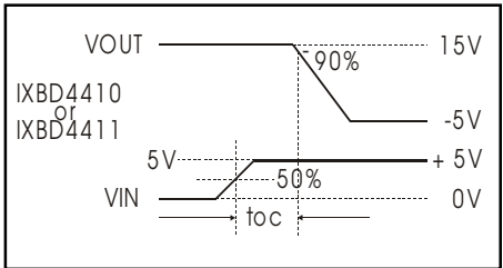
Fig. 1b Overcurrent Delay
