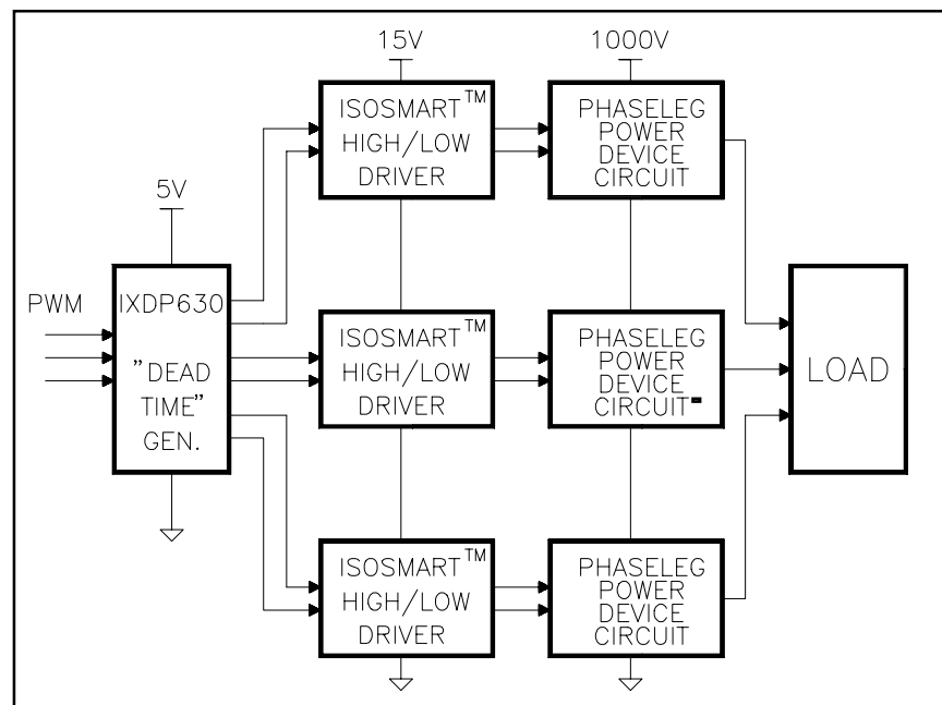
Fig. 9: Typical 3-phase motor control system block diagram
