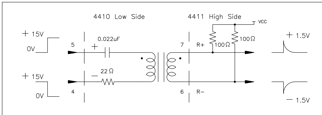
Fig. 13: Transmitter/Receiver Waveforms
