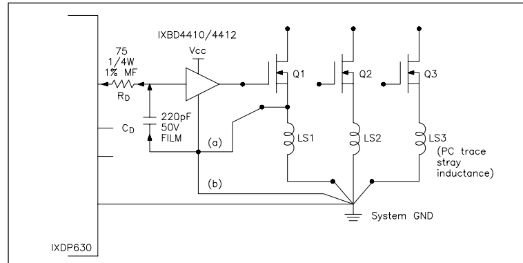
Fig. 11: Potential layout problems that create functional problems
