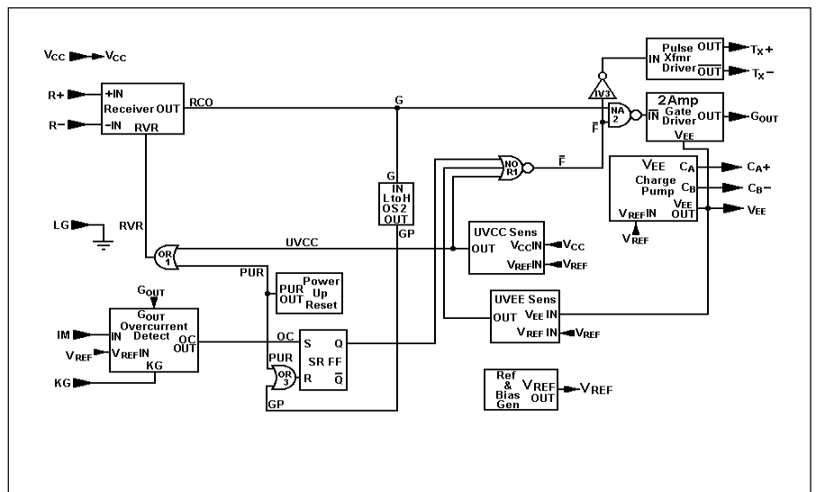
Fig. 4: IXBD4411, high-side driver block diagram
