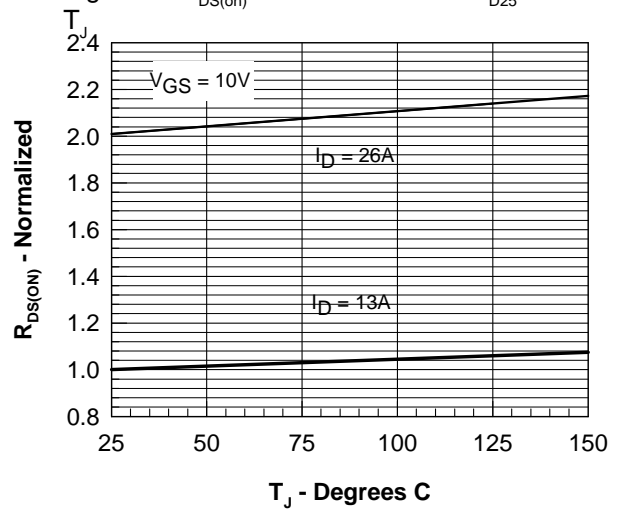
Figure 6. R_{DS(on)} normalized to 0.5 I_{D25} value vs. T_J
