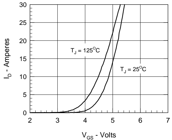
Figure 4. Admittance Curves
