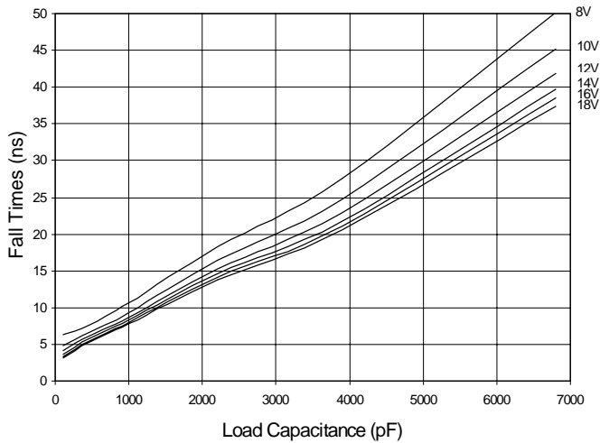
Fig. 7 Output Fall Times vs. Load Capacitance
