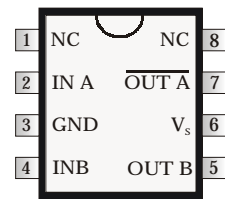
8 Lead PDIP (PI) 8 Pin SOIC (SI) IXDF402
