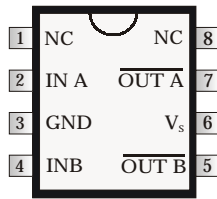
8 Lead PDIP (PI) 8 Pin SOIC (SI) IXDI402
