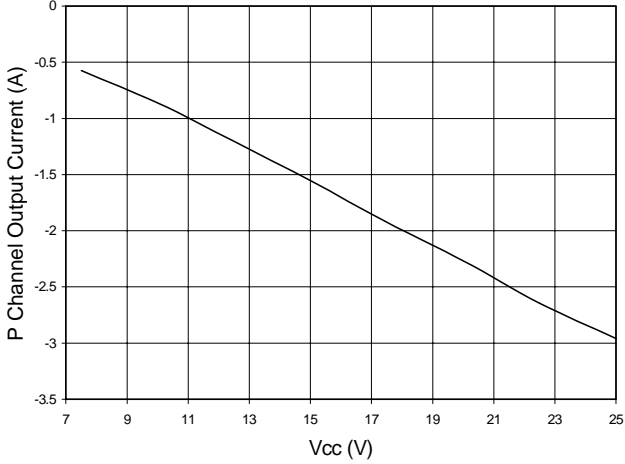
Fig. 23 Vcc vs. P Channel Output Current
