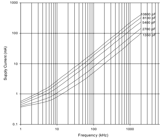
Fig. 10 Supply Current vs. Frequency V cc = 18V
