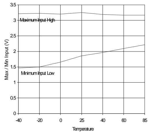
Fig. 8 Max / Min Input vs. Temperature
