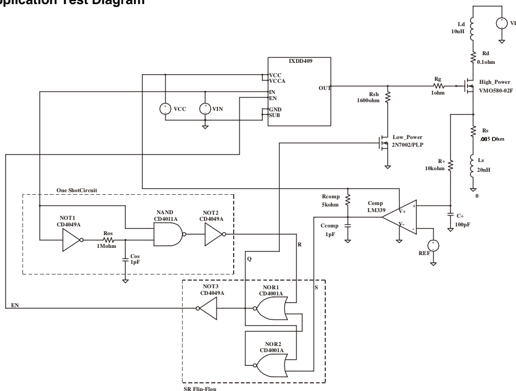
Figure 26 - Application Test Diagram
