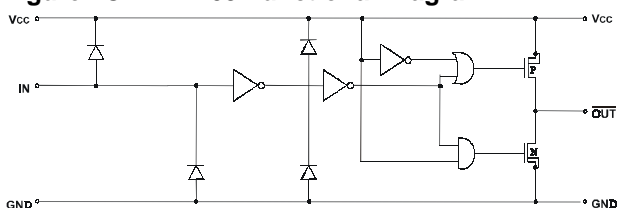
Figure 1C - IXDI409 Functional Diagram
