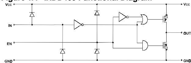
Figure 1B - IXDN409 Functional Diagram
