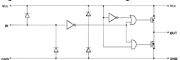
Figure 1C - IXDI409 Functional Diagram
