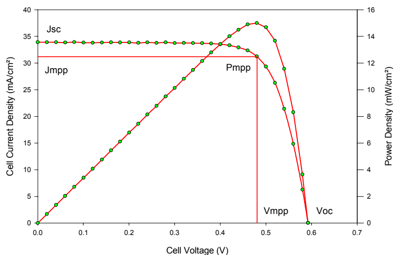
IXOLAR™ XOD - 15 (measured at 100 mW/cm 2 , AM 1.5, 25°C)
