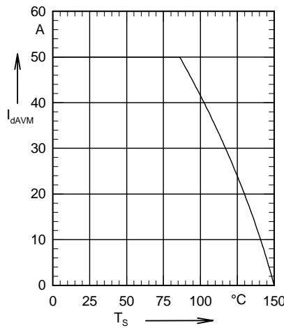
Fig. 2 Maximum forward current at heatsink temperature T_S .
