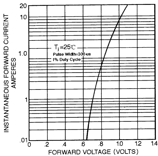
FIG. 3-TYPICAL FORWARD CHARACTERISTICS PER ELEMENT
