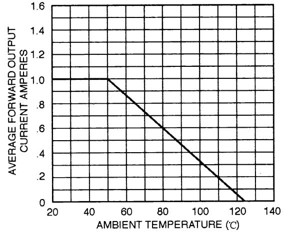
FIG. 2-TYPICAL FORWARD OUTPUT CURRENT DERATING CURVE
