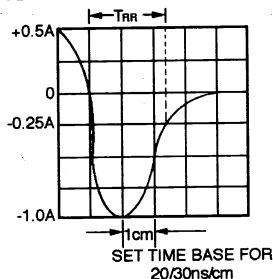
FIG. 1 - TEST CIRCUIT DIAGRAM AND REVERSE RECOVERY TIME CHARACTERISTICS
