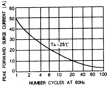
FIG. 1-MAXIMUM NON-REPETITIVE FORWARD SURGE CURRENT - PER ELEMENT
