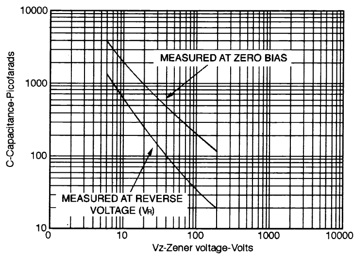
FIGURE 3 – Typical Capacitance Vs. Zener Voltage
