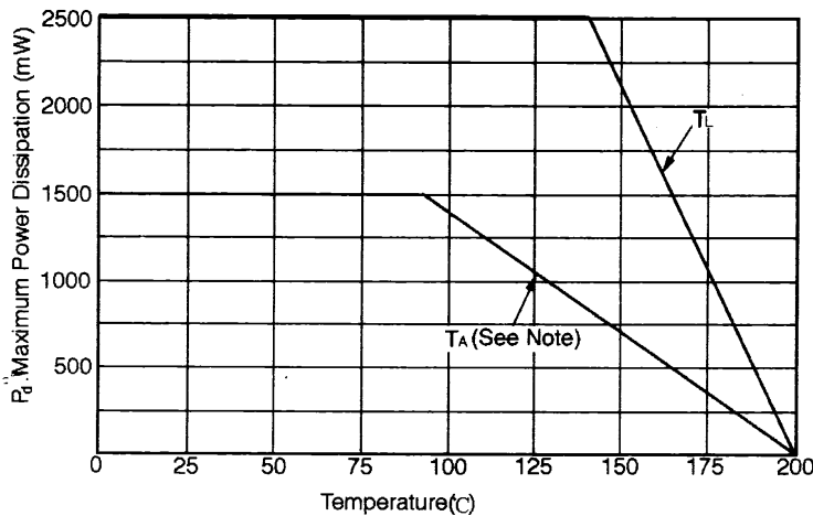
FIGURE 1 – Power Derating Curve
