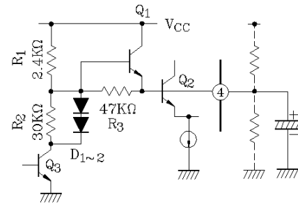
Fig. 1 Internal circuit of pin ④
