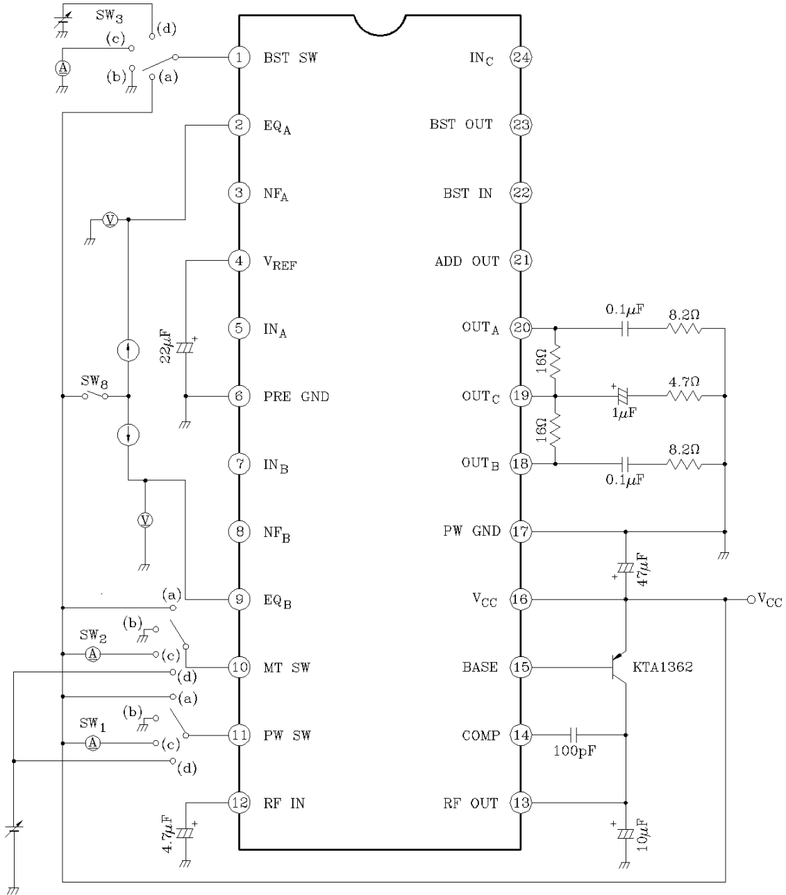
TEST CIRCUIT 1
