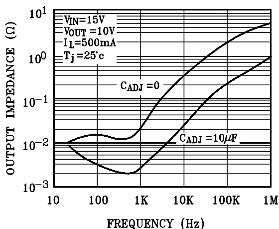
Output Impedance
