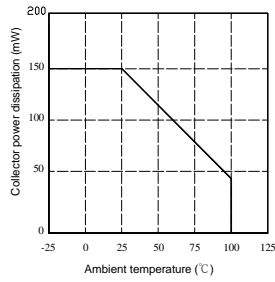
Collector power dissipation Vs. Ambient temperature
