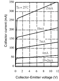
Collector current Vs. Collector-Emitter voltage
