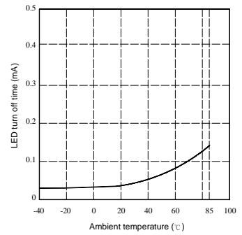
LED turn off time Vs. Ambient temperature
