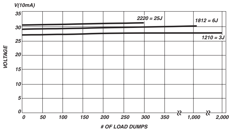
FIGURE 6. REPETITIVE LOAD DUMP PULSING AT RATED ENERGY
