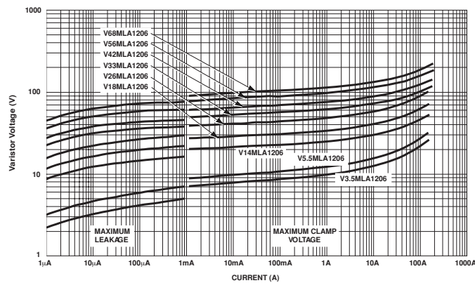
FIGURE 8. LIMIT V-I CHARACTERISTIC FOR V3.5MLA1206 TO V68MLA1206
