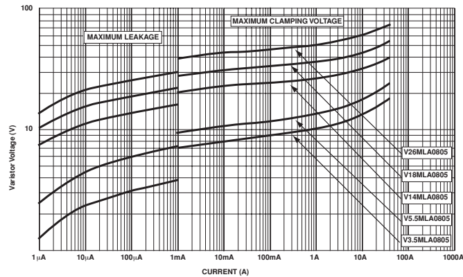
FIGURE 7. LIMIT V-I CHARACTERISTIC FOR V3.5MLA0805 TO V26MLA0805
