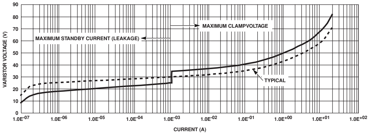
FIGURE 5. V-I CHARACTERISTICS
