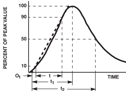
FIGURE 2. PEAK PULSE CURRENT TEST WAVEFORM FOR CLAMPING VOLTAGE
