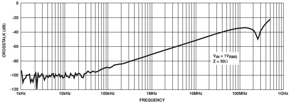
FIGURE 11. ADJACENT CHANNEL CROSSTALK
