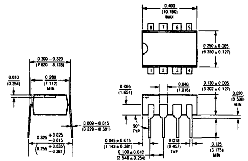
N8 Package 8 Lead Plastic
