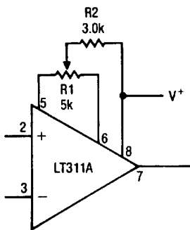
Offset Balancing
