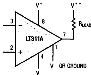
Driving Load Referenced To Positive Supply
