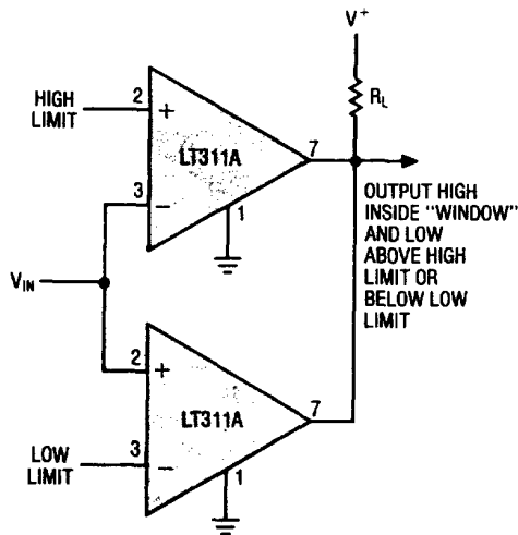
Window Detector
