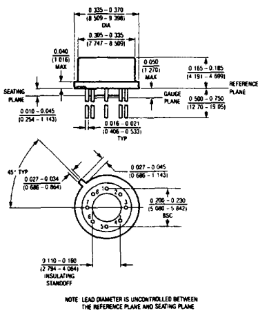
H Package Metal Can
