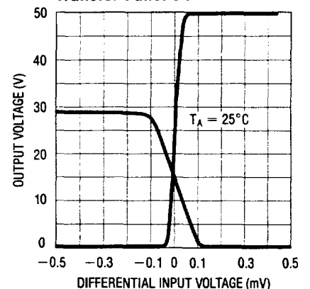
Transfer Function
