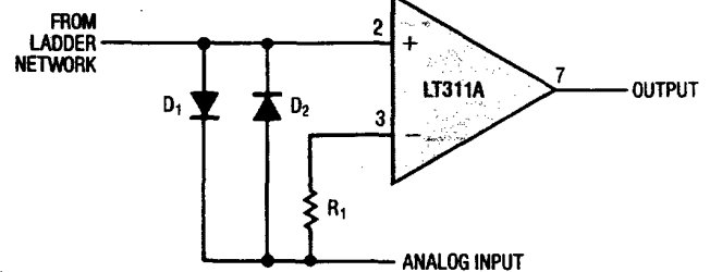
Using Clamp Diodes To Improve Frequency Response*
