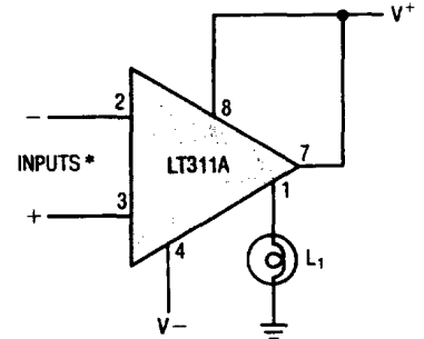
Driving Ground Referred Load
