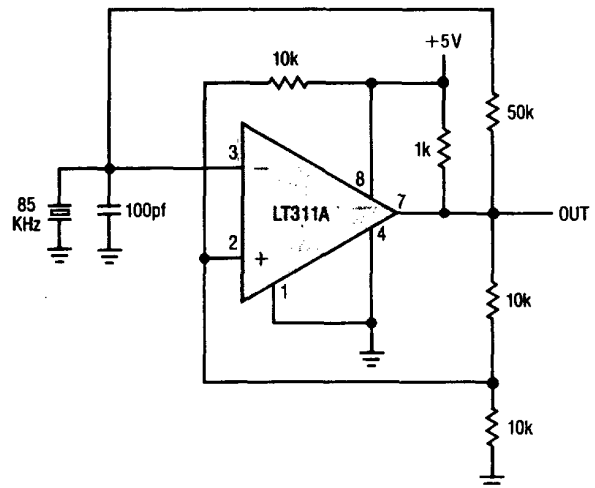
Crystal Oscillator
