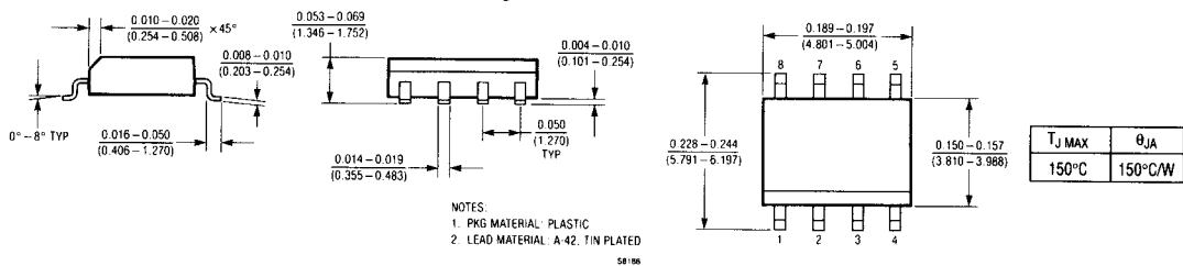
S8 Package, 8-Lead Plastic SOIC
