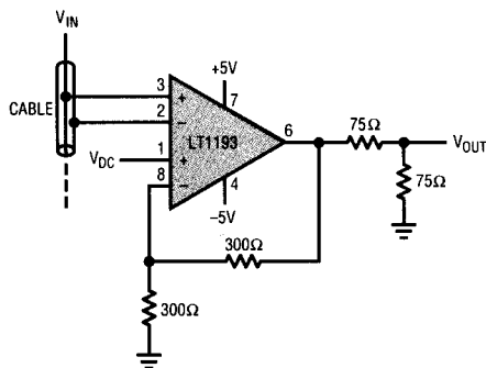
Cable Sense Amplifier for Loop Through Connections with DC Adjust
