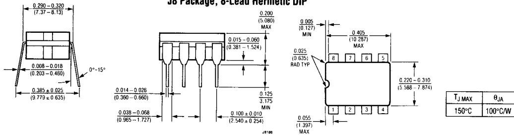
N8 Package, 8-Lead Plastic DIP
