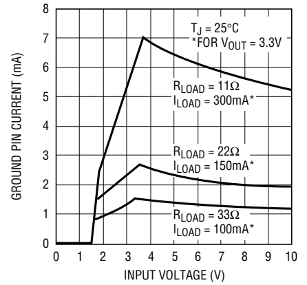
LT1521-3.3 Ground Pin Current
