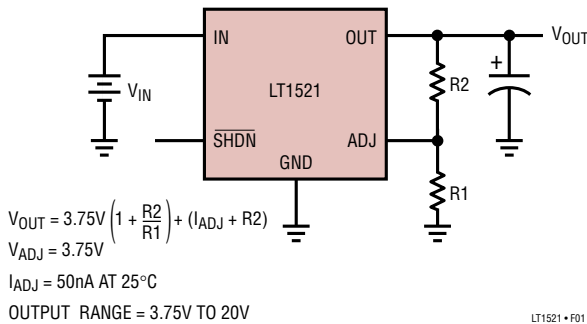
Figure 2. Adjustable Operation
