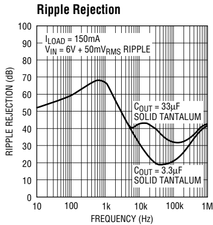
LT1521 • TPC31
