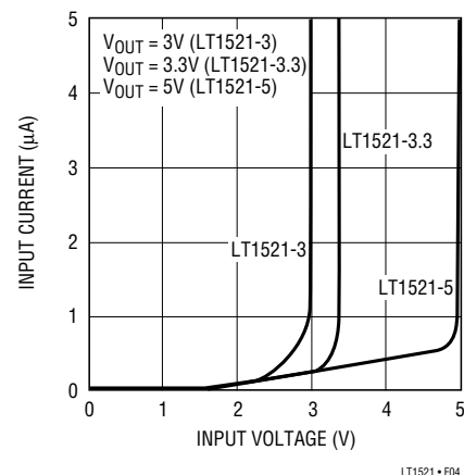
Figure 4. Input Current
