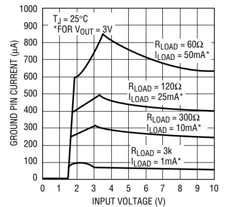
LT1521-3 Ground Pin Current
