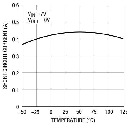
Current Limit
