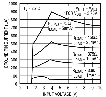
LT1521 Ground Pin Current
