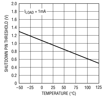
Shutdown Pin Threshold (On-to-Off)
