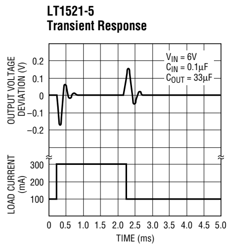
LT1521 • TPC34
