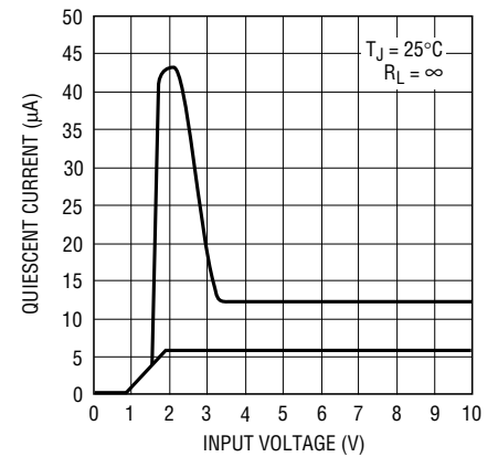
LT1521-3.3 Quiescent Current
