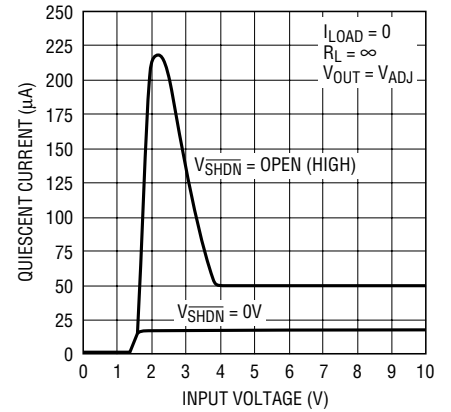
LT1529 Quiescent Current
