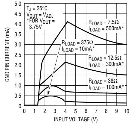
LT1529 GND Pin Current
