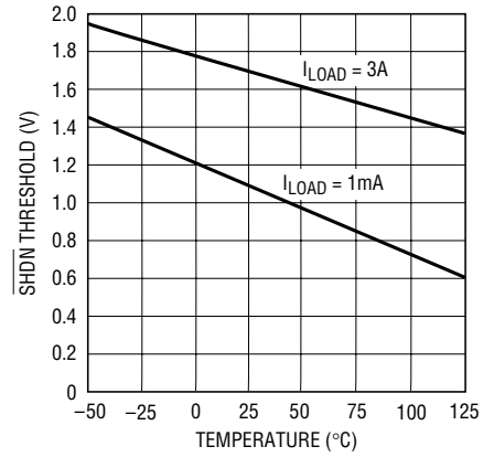
SHDN Pin Threshold (Off-to-On)
