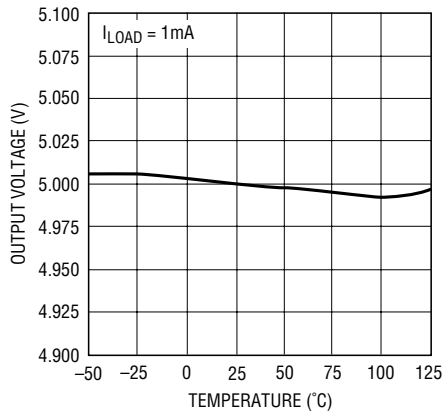
LT1529-5 Output Voltage
