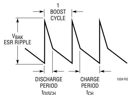
Figure 3. V_{BAK} Ripple
