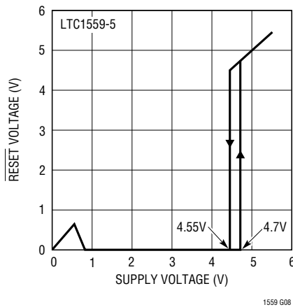
RESET Output Voltage vs Supply Voltage
