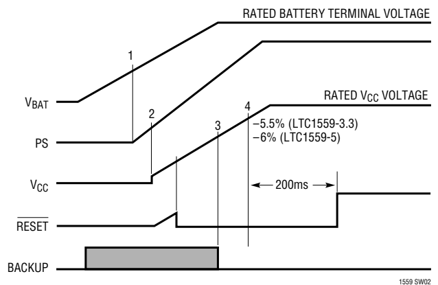
Cold Power Boot-Up (Main Battery Replaced/Turned On)
