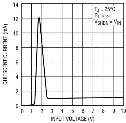
LT1963-2.5 Quiescent Current
