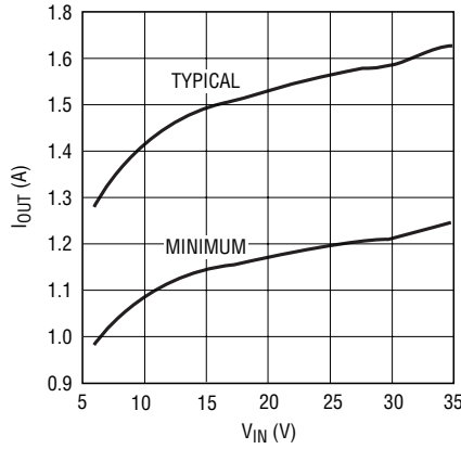
High Voltage Regulator Maximum Load Current, L = 33μH
