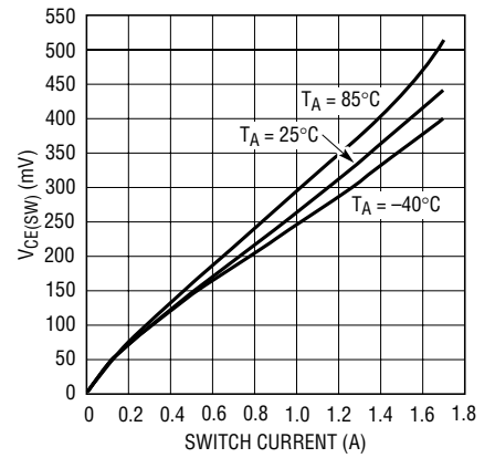
High Voltage Regulator Switch Voltage Drop
