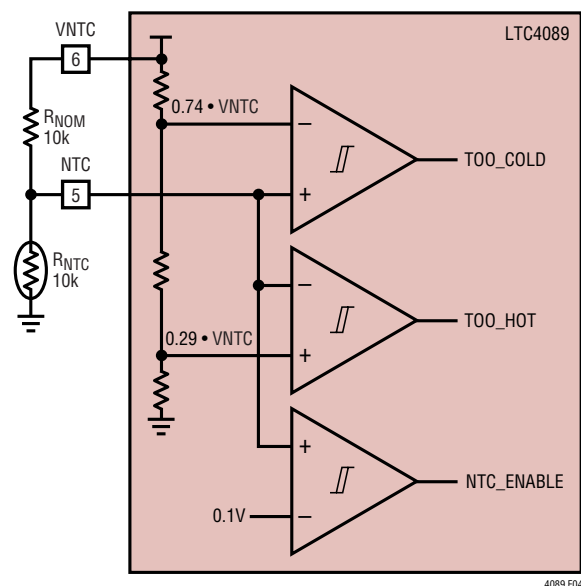
Figure 4. NTC Circuit
