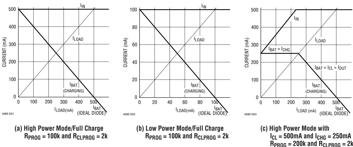
Figure 2. Input and Battery Currents as a Function of Load Current
