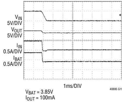
Input Disconnect Waveforms
