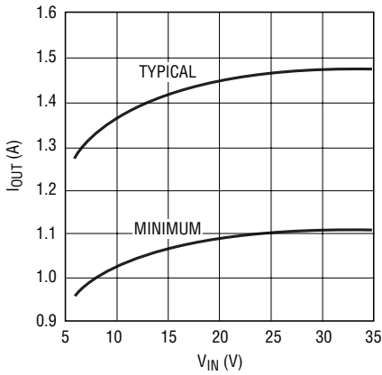
High Voltage Regulator Maximum Load Current, L = 10μH
