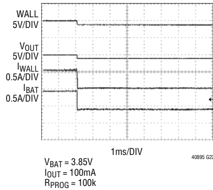
Wall Disconnect Waveforms
