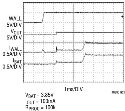
Wall Connect Waveforms
