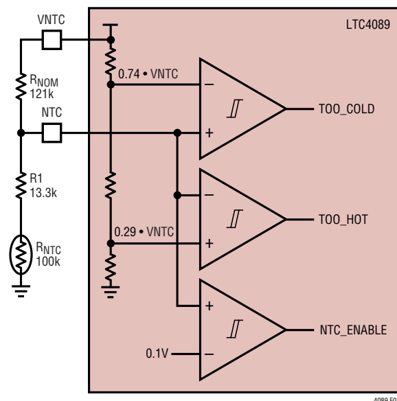
Figure 7. Modified NTC Circuit
