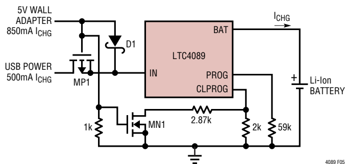
Figure 5. USB or 5V Wall Adapter Power
