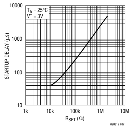
Figure 7. Start-Up Time
