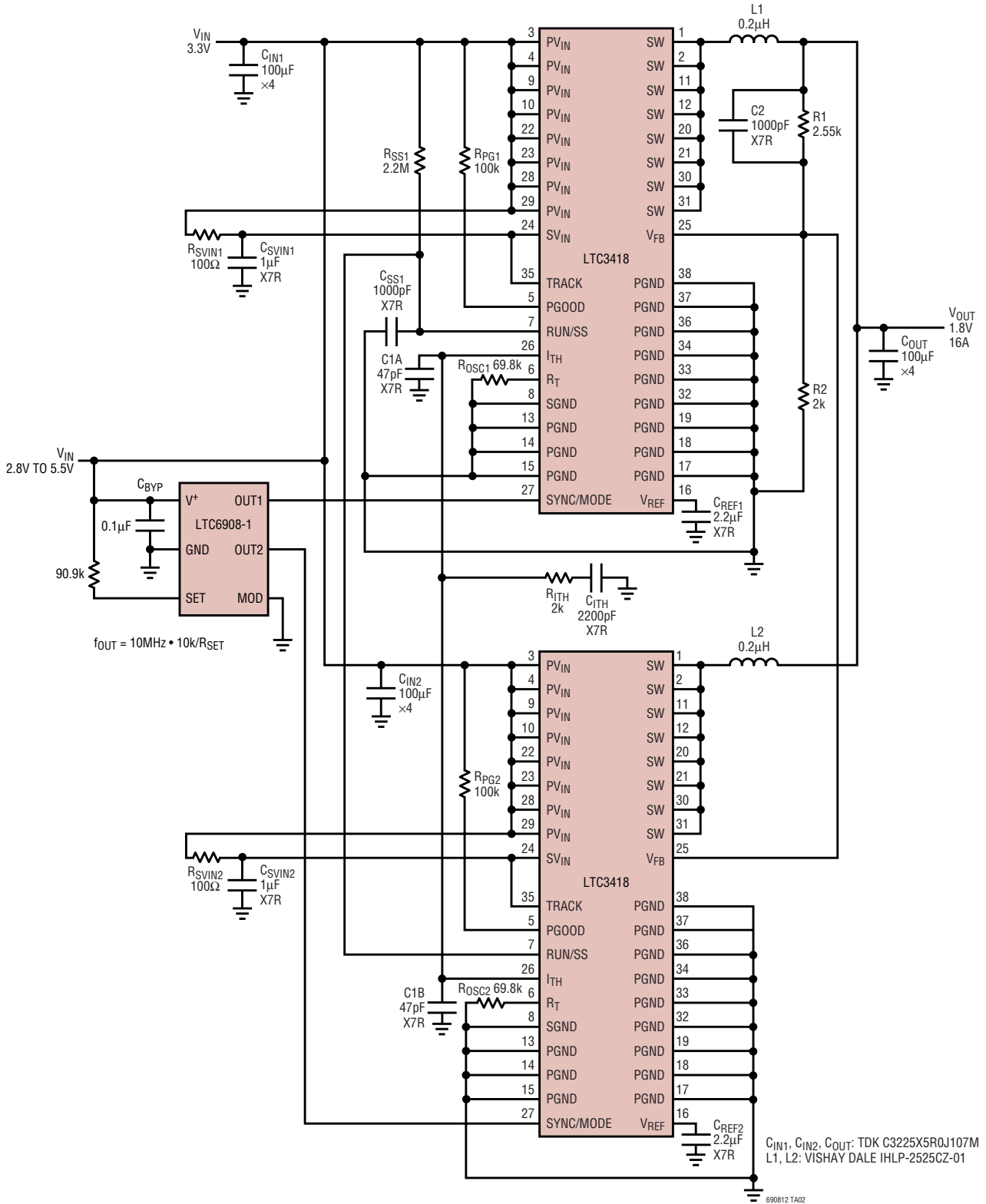
Figure 8a. 1.1MHz, 1.8V/16A Step-Down Regulator
