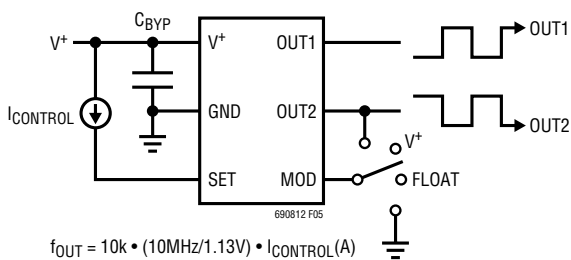
Figure 5. Current Controlled Oscillator
