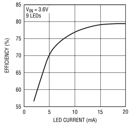
Conversion Efficiency
