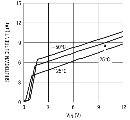
Shutdown Current ( V_{CTRL} = 0\text{V} )
