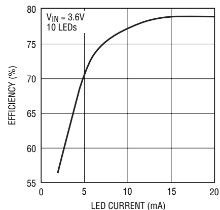
Conversion Efficiency
