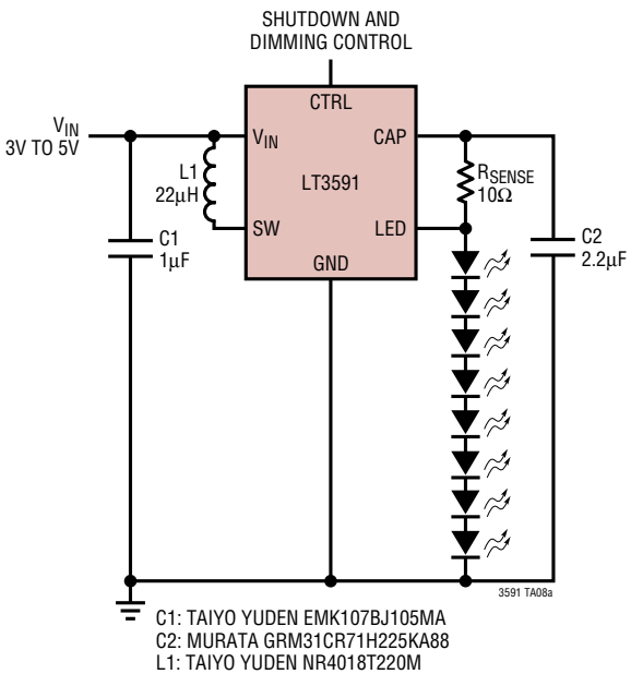
Li-Ion Driver for Eight White LEDs
