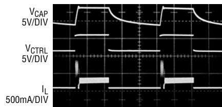
Transient Response
