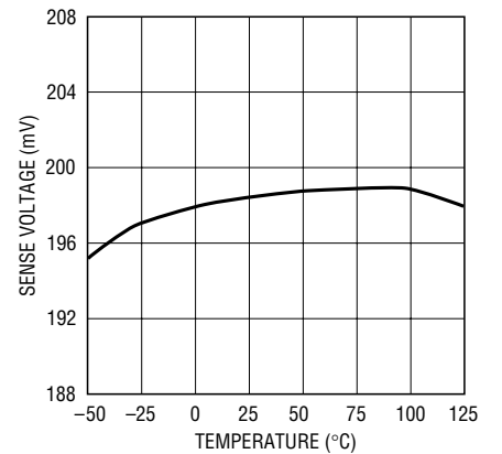
Sense Voltage ( V_{CAP} - V_{LED} ) vs Temperature
