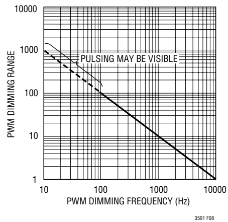
Figure 8. Dimming Range vs Frequency
