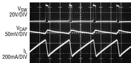
Switching Waveform
