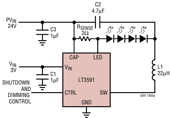
24V to Four White LEDs at 100mA
