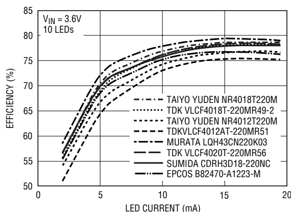
Figure 3. Efficiency Comparison of Different Inductors
