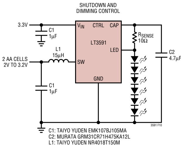
Figure 10. 2 AA Cells to Six White LEDs
