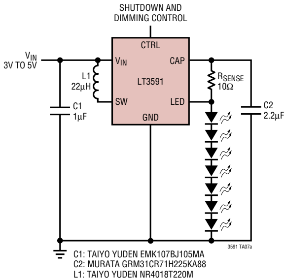
Li-Ion Driver for Seven White LEDs
