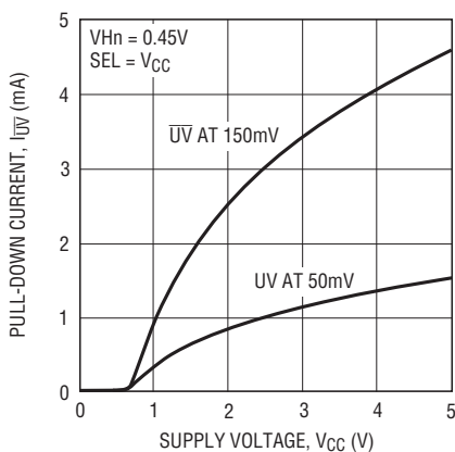
\overline{\text{UV}} , I_{\text{SINK}} vs V_{CC}
