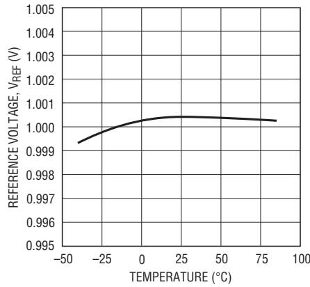
Buffered Reference Voltage vs Temperature
