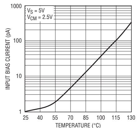
LTC6087 Input Bias Current vs Temperature
