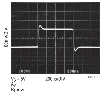
Small-Signal Response
