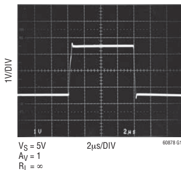
Large-Signal Response
