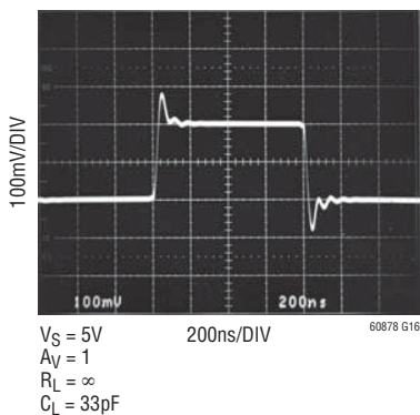
Small-Signal Response
