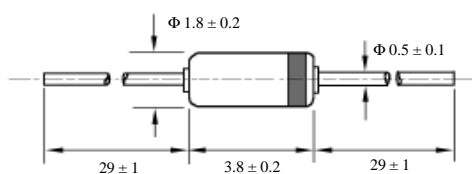
DO-35 (mm)
