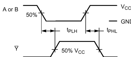
Figure 4. Switching Waveforms
