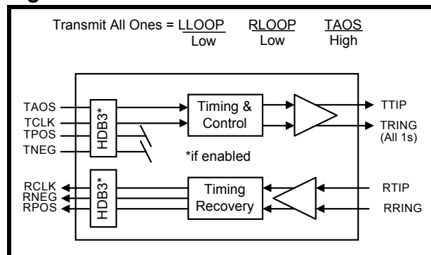
Figure 3: Transmit All Ones
