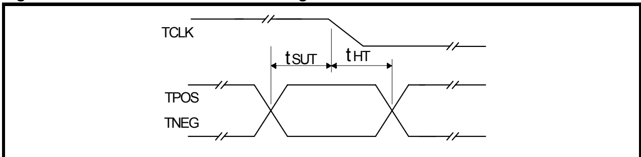
Figure 12: LXT317 Transmit Clock Timing
