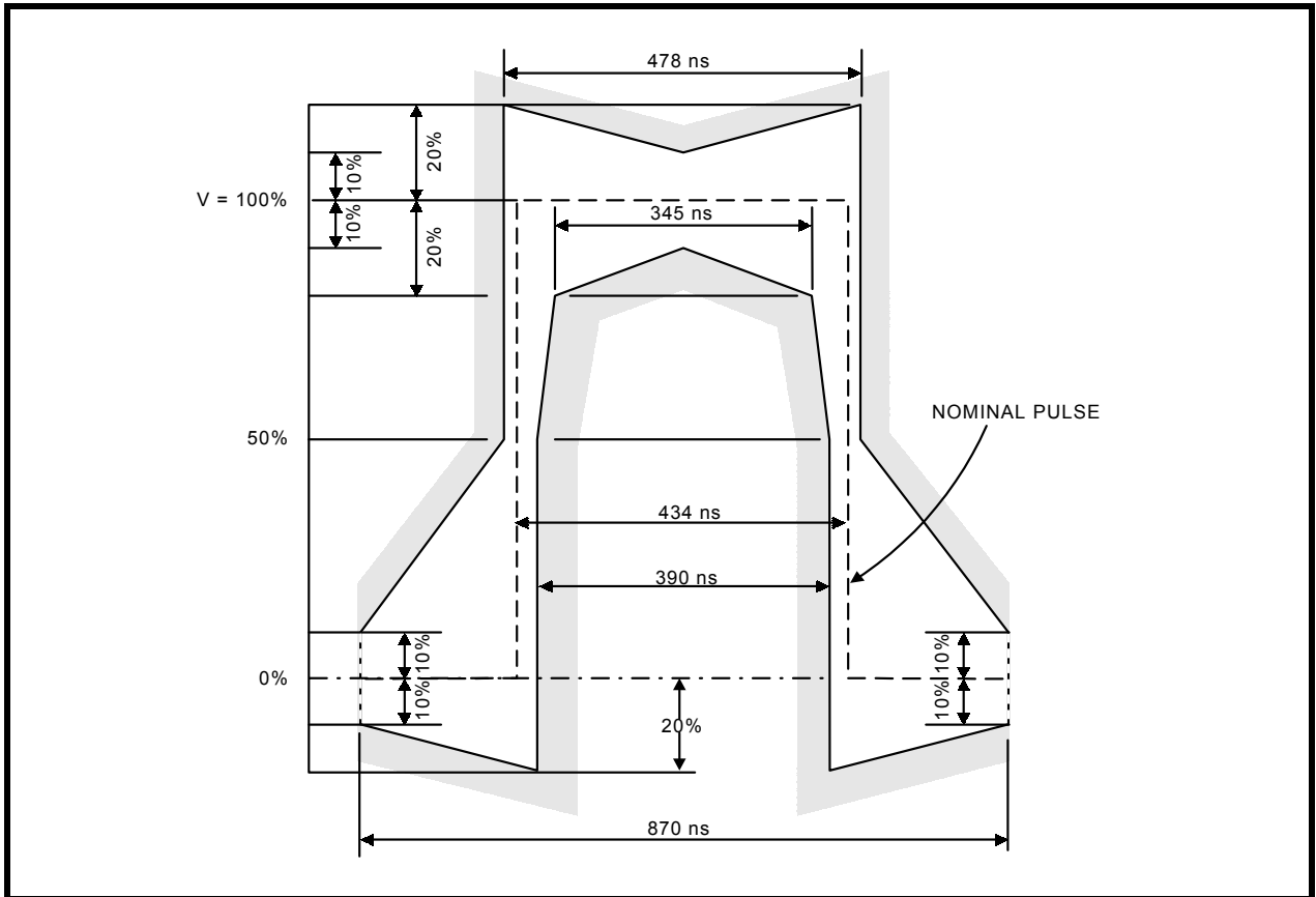
Figure 11: 1.152 MHz Pulse Mask
