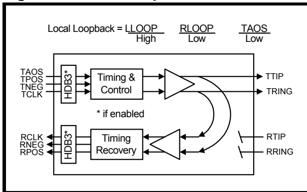
Figure 6: Local Loopback
