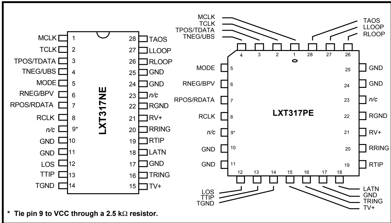
Figure 1: LXT317 Pin Assignments
