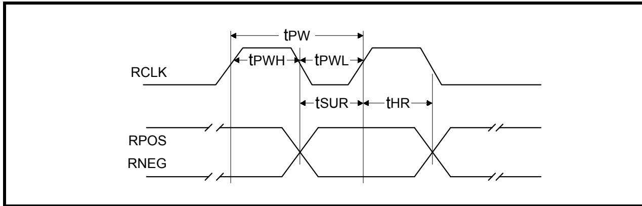
Figure 13: LXT317 Receive Clock Timing
