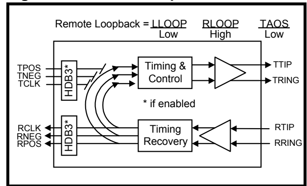
Figure 7: Remote Loopback
