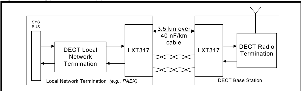
Figure 9: Typical DECT Application
