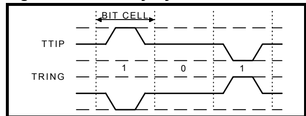
Figure 2: 50% Duty Cycle Transmit Pulse
