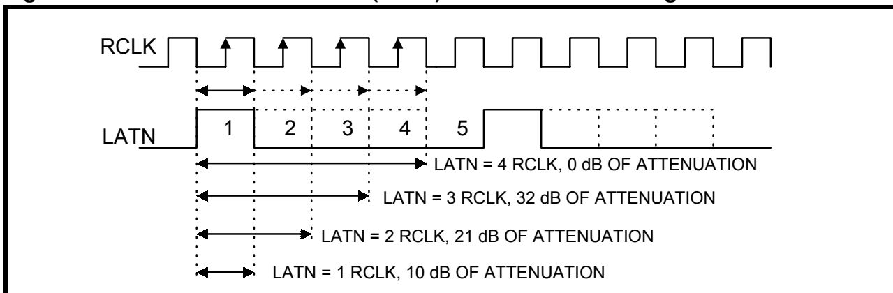
Figure 5: LXT317 Line Attenuation (LATN) Pulse Width Encoding
