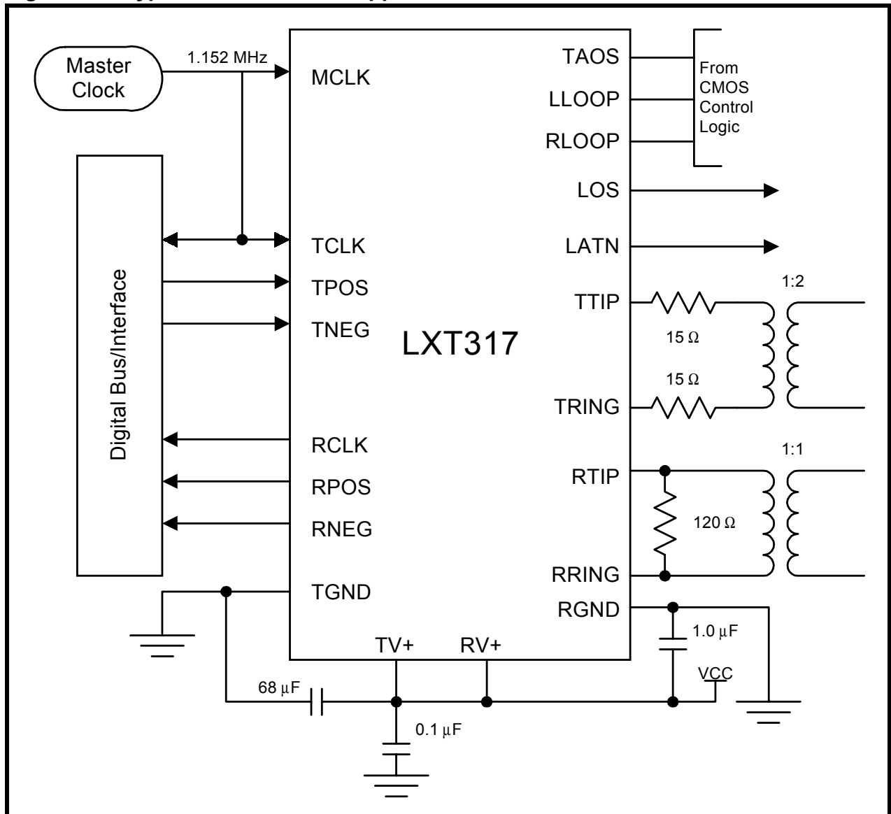
Figure 10: Typical LXT317 DECT Application
