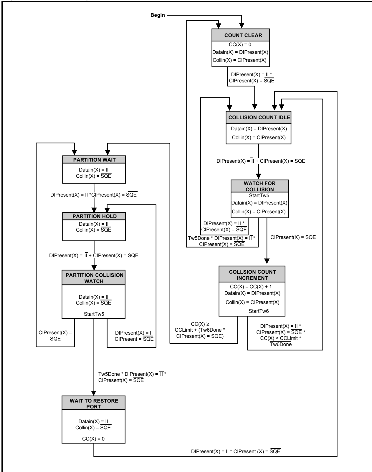
Figure 3: Partitioning State Machine
