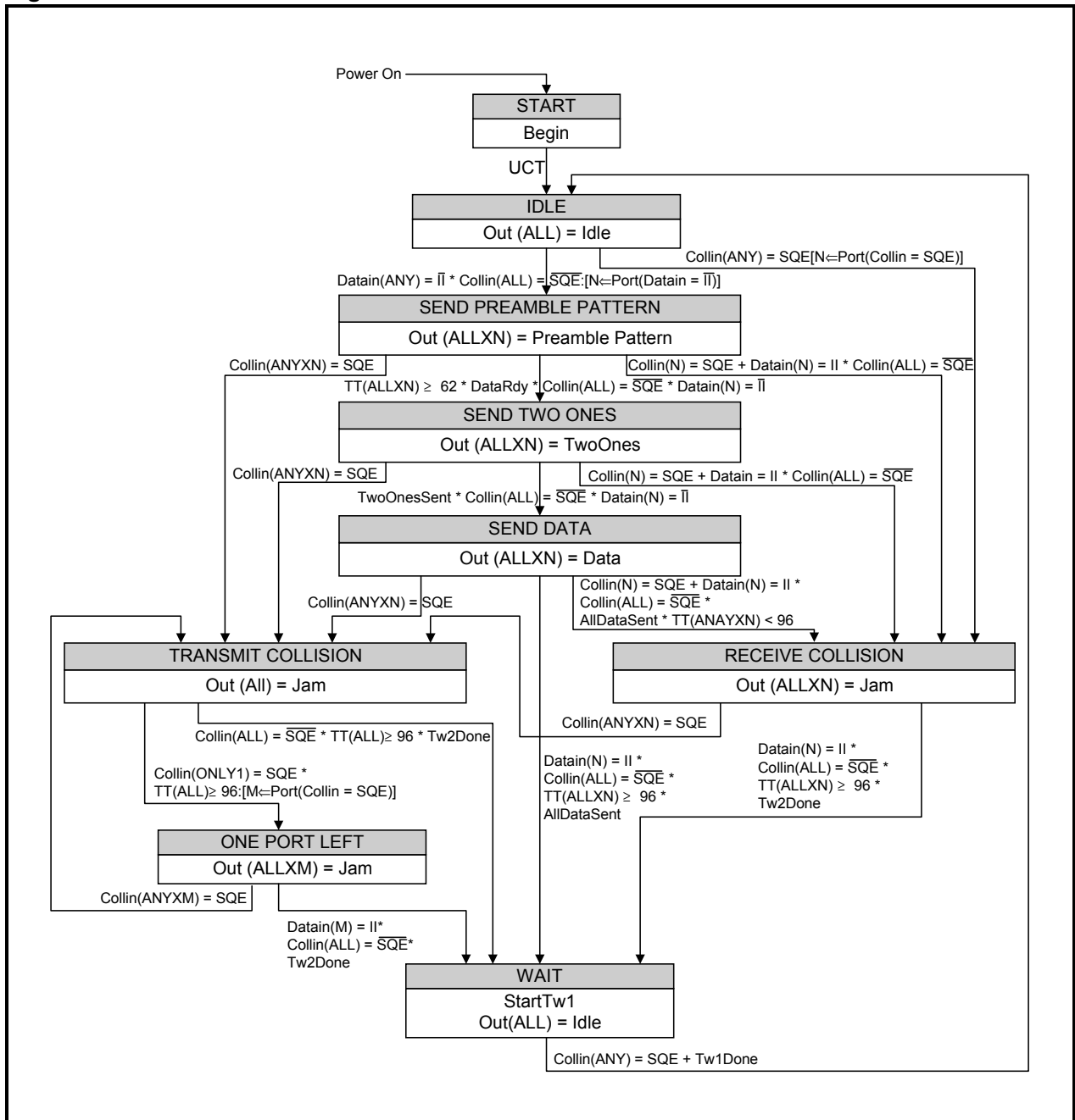
Figure 2: Global State Machine
