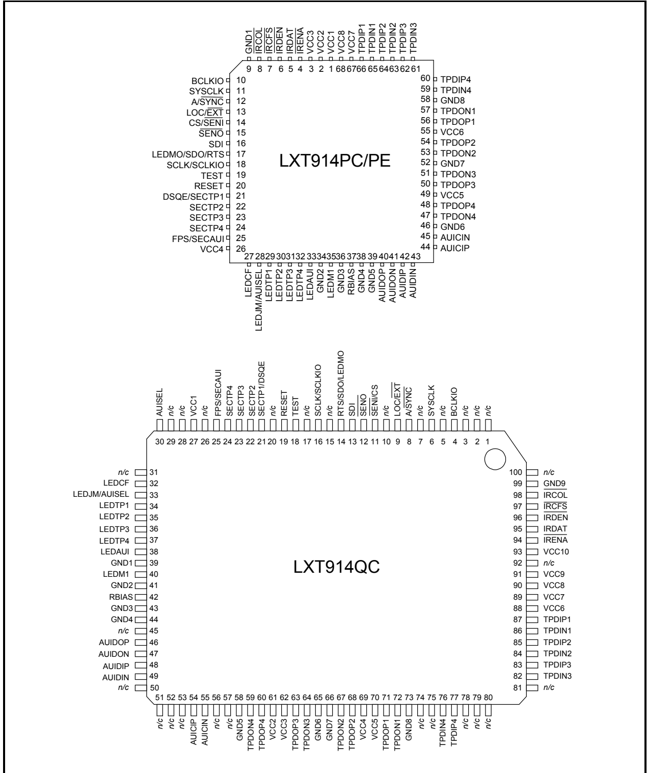
Figure 1: LXT914 Pin Assignments
