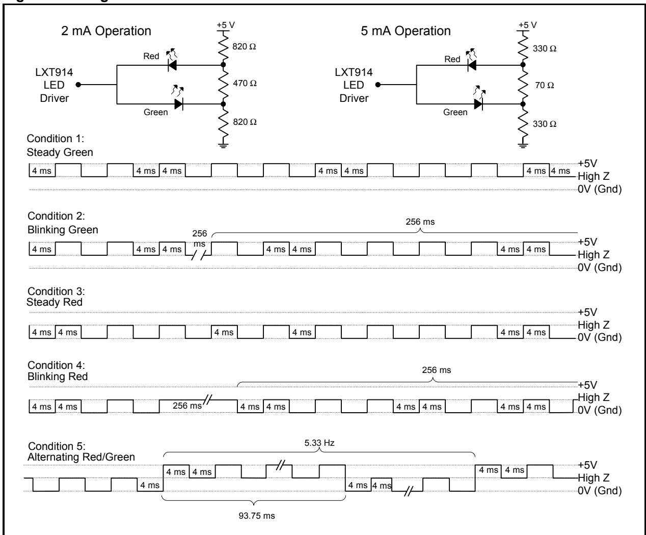
Figure 4: Integrated LED Driver Indications
