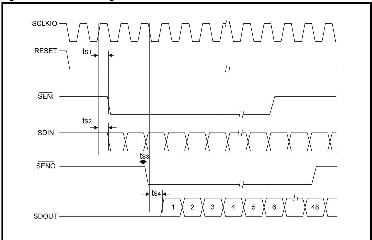
Figure 7: Serial Port Timing
