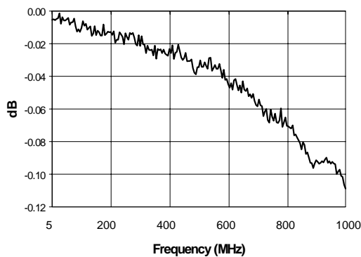
Amplitude Unbalance
