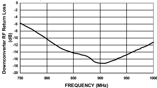
RF Return Loss Temp = 25°C, V_{DD} = 2.7V, I_{DD} = 15 mA
