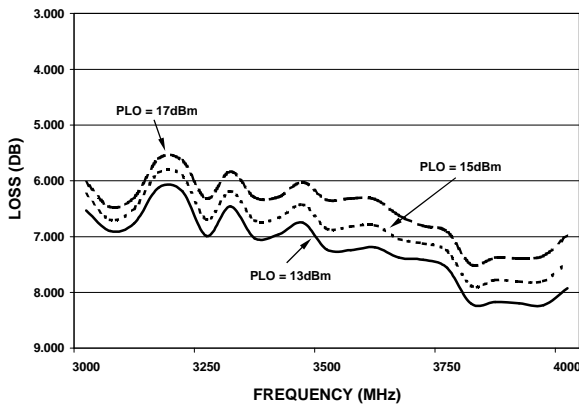
Conversion Loss
